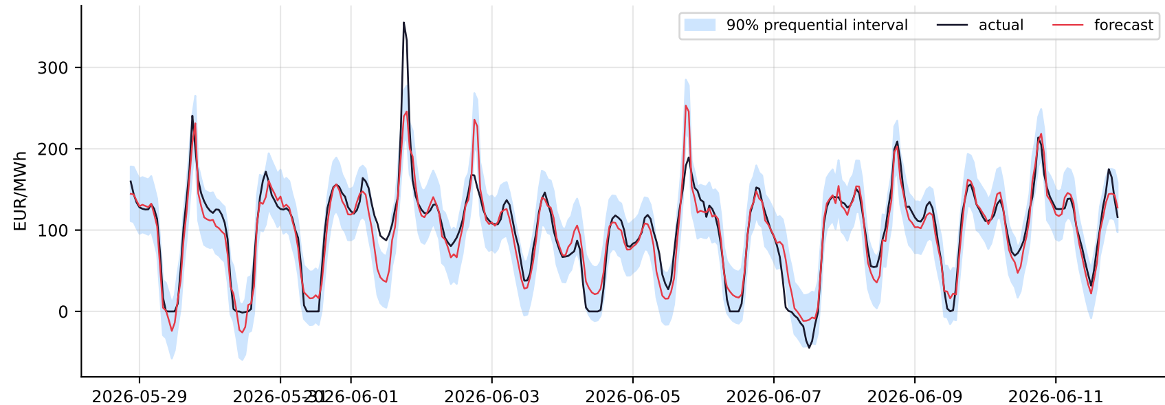
Strictly prequential conformal intervals -- last 14 days
